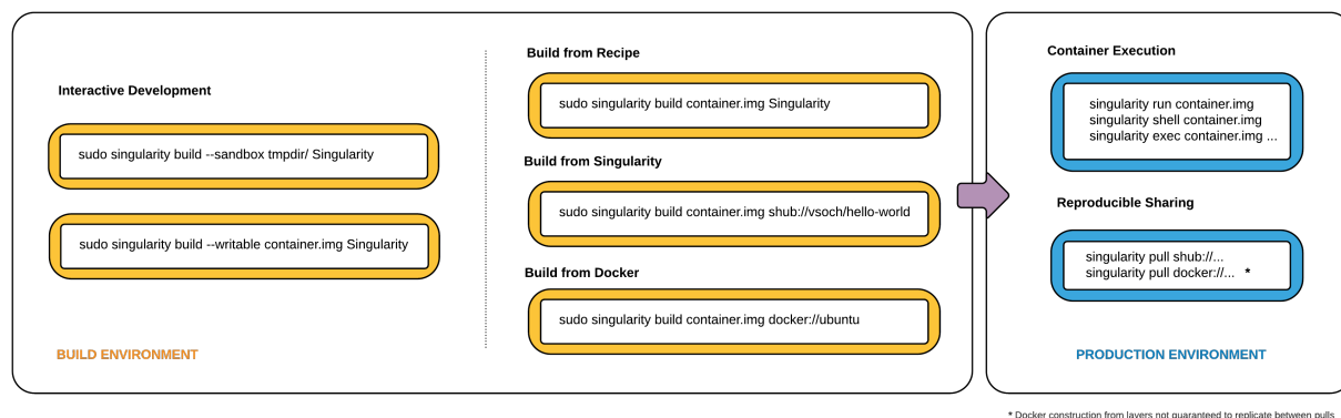
Fig. 1: Singularity Workflow
